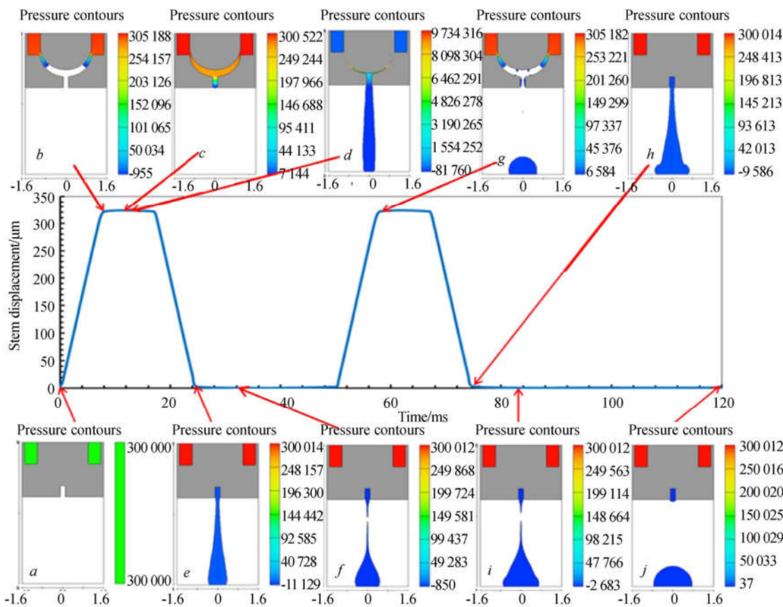
图 7 阀杆位移曲线及关键位置压力云图 Fig. 7 Displacement curve of stem and pressure cloud diagram of key position
