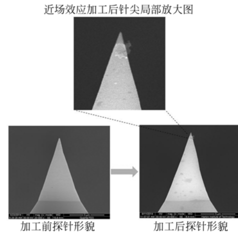
(a) 激光复合微纳探针加工纳结构后的探针 SEM 图 (a) SEM images of AFM probe before and after machining nanostructure combined with laser
