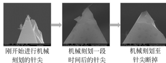
(b) 机械刻划后的探针 SEM 图 (b) SEM images of AFM probe after machining nanostructure by mechanical characterization
