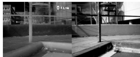
(b) SURF
