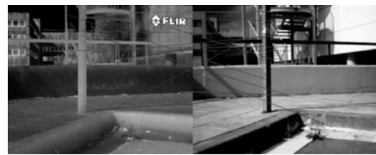
(a) MM-SURF
