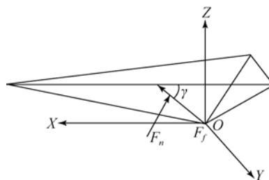
图1 刻划刀受力示意图 Fig.1 Force diagram of ruling tool
